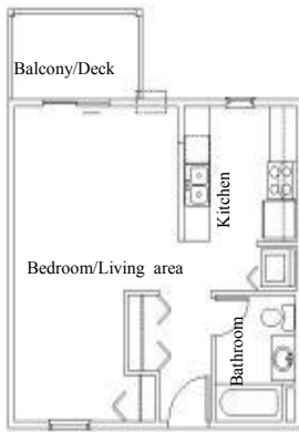
Pioneer 485 Sq. Feet Bedroom /living area 21'4"x15'2"
